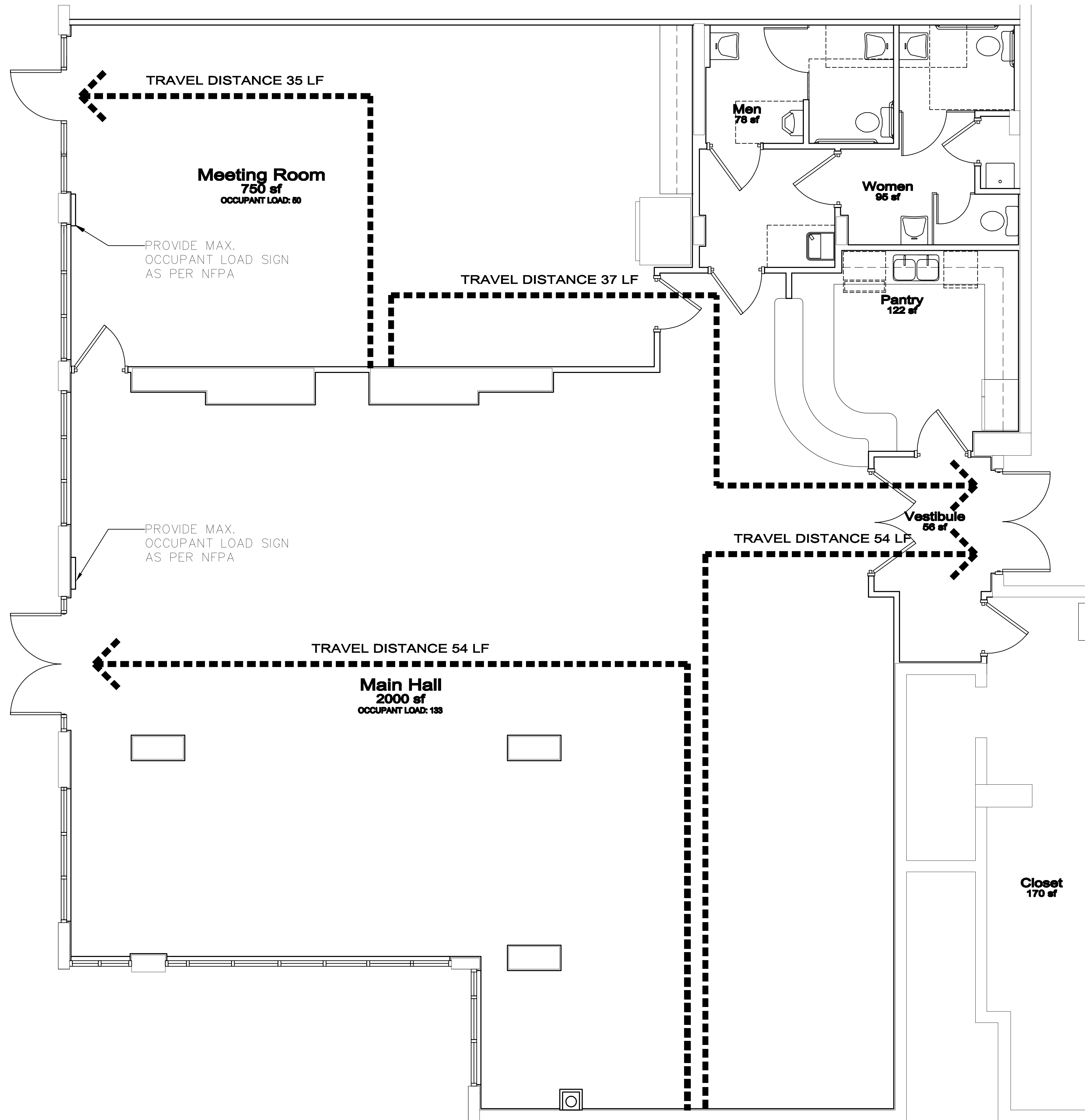
1 Fire Plan F-1.1 SCALE: 1/4" = 1'-0"
